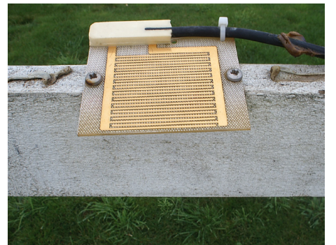
Unpainted flat plate wetness sensors in and out of a crop
